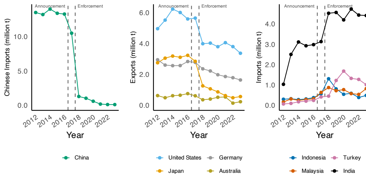
Figure A1: Plastic and Paper Scrap Imports and Exports Over Time
