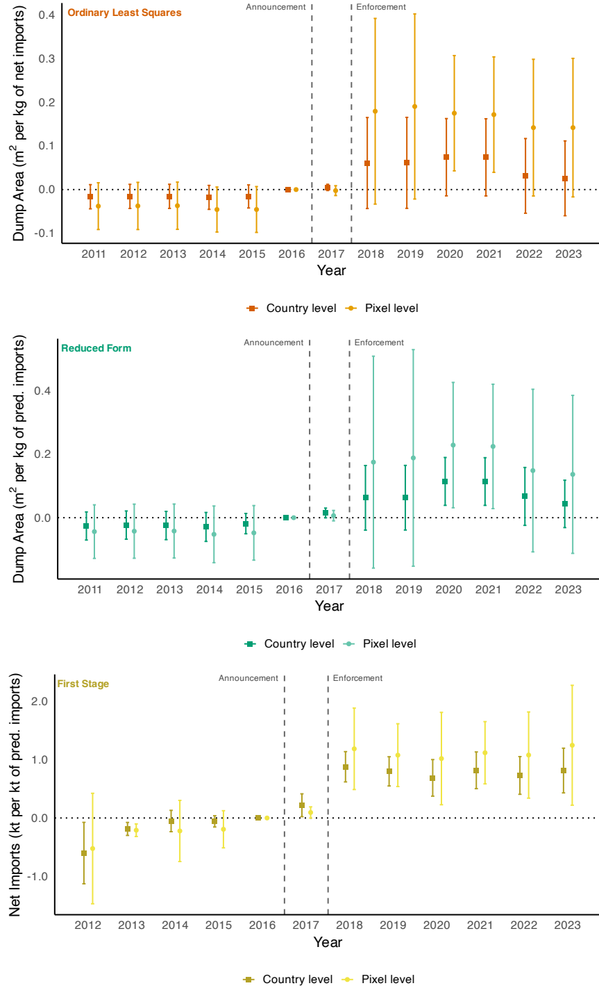
Figure A8: Effect of Change in Net Imports on Open Dump Area, Event Study Version
