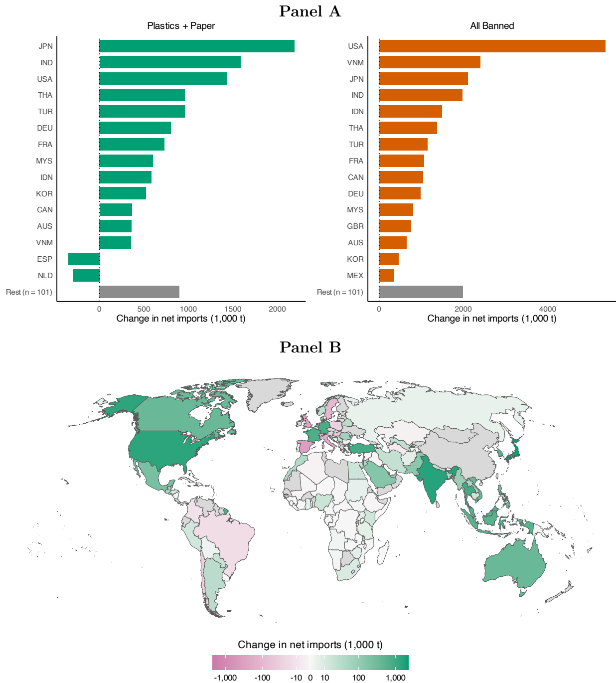
Figure A7: Change in Net Imports Following China's National Sword Policy
