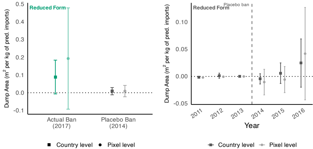
Figure A11: Effect of Change in Net Imports on Open Dump Area, Placebo Ban Analysis
