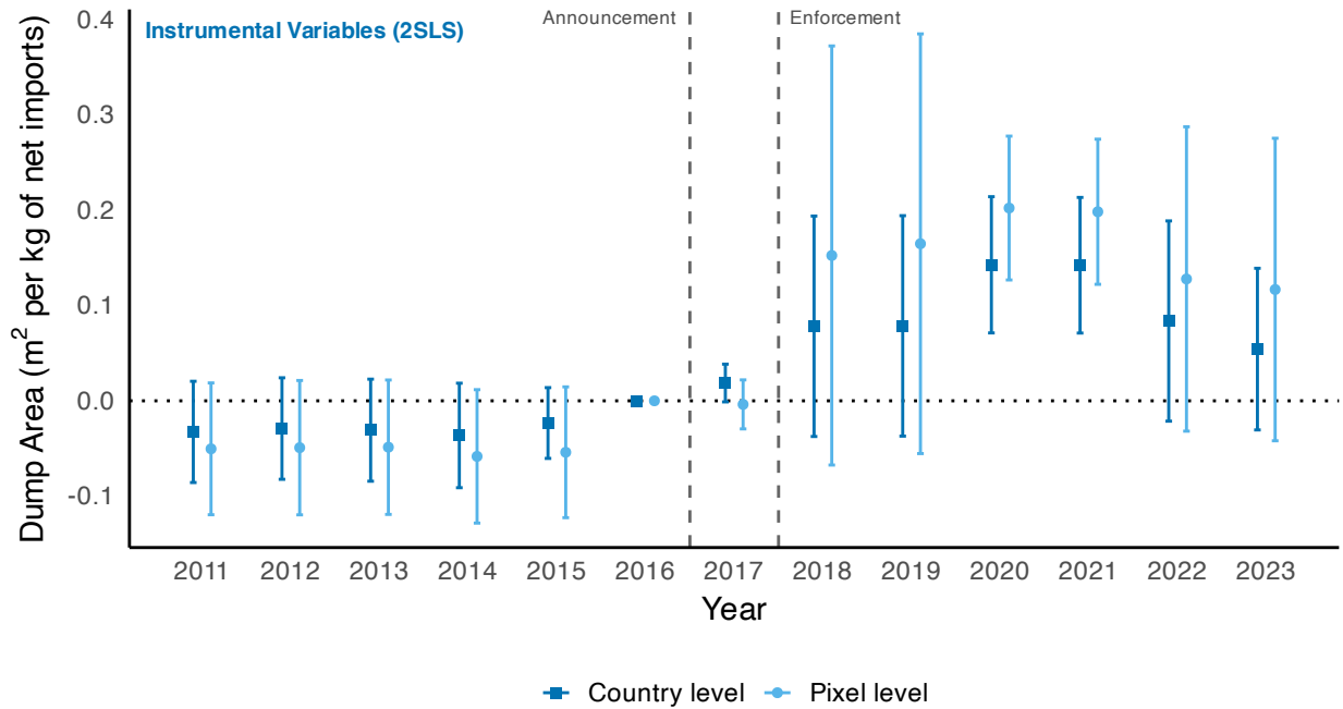
Figure 8: Effect of Change in Net Imports on Open Dump Area, Event Study Version
