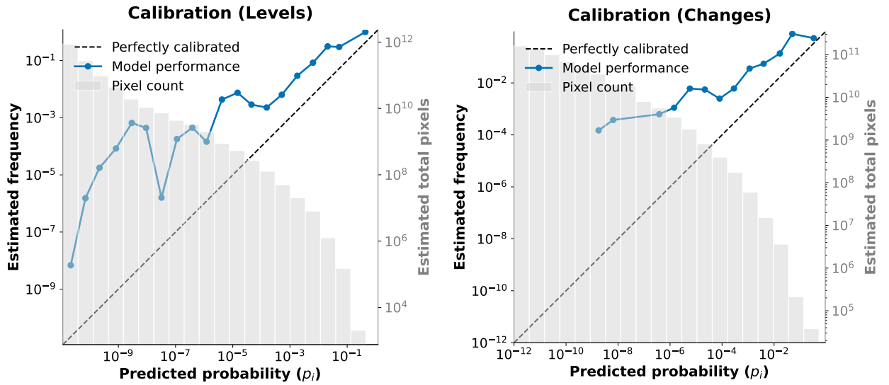
Figure 3: Model Calibration
