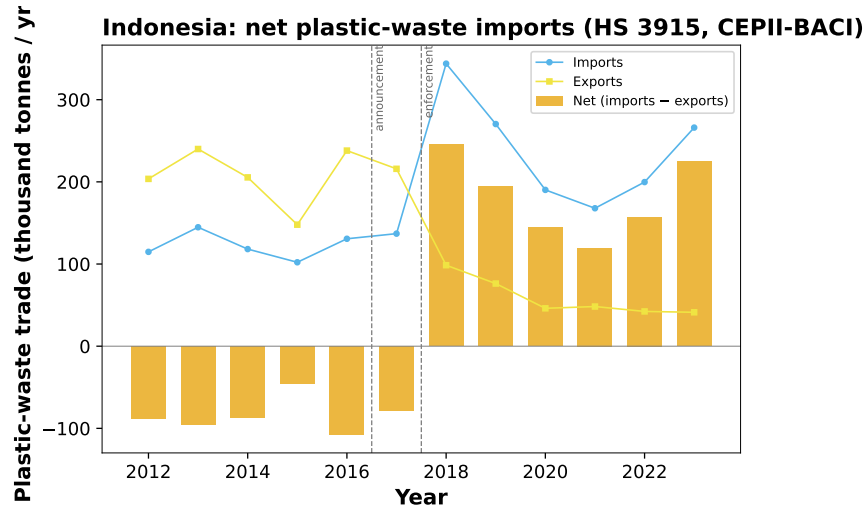
Figure A16: Indonesia: Net Imports of Plastic Waste Around the China Ban
