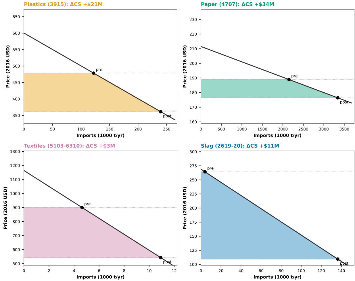
Figure A17: Indonesia consumer-surplus gain from the supply shock induced by the 2018 China waste-import ban, by category of banned waste. Each panel reads the surplus change off the observed pre (2012–16) \rightarrow post (2018–23) price and quantity changes. Points mark pre/post (quantity, price); the solid line is the revealed linear demand; the shaded area is the realized surplus change. Constant 2016 prices deflated using Indonesian CPI converted to 2016 USD.
